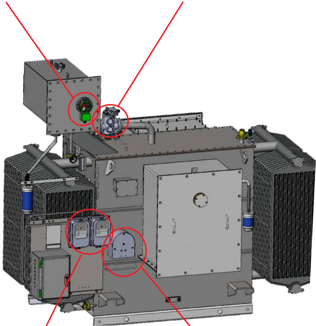
Magnetic Oil Gauge
