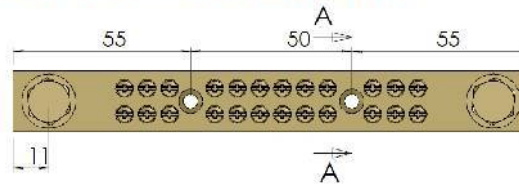
TYPICAL 12 POLE/WAY WITH 50mm MOUNTING CENTRES
